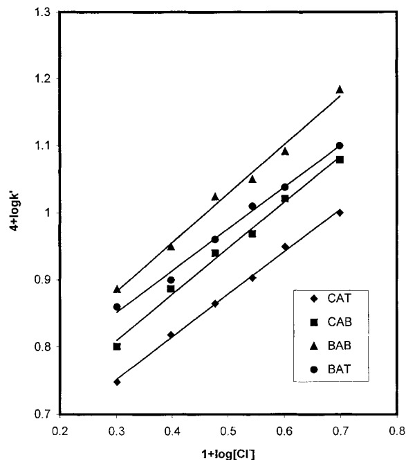
Figure 4. Plot of \log[\text{Cl}^-] vs \log k'
