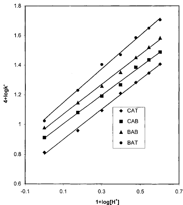
Figure 3. Plot of \log[\text{H}^+] vs \log k' at 308 K
