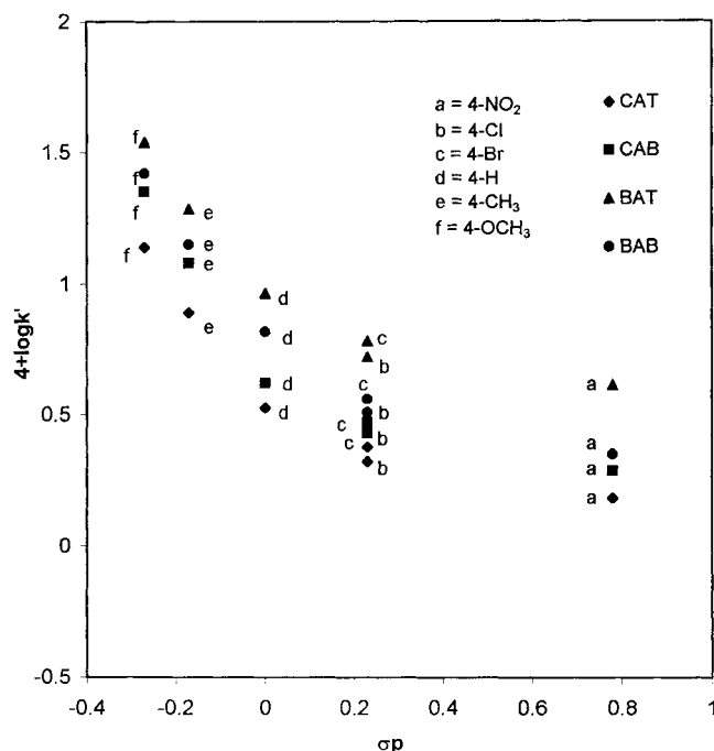
Figure 5. Hammett plot ( 4 + \log k' vs \sigma_p ) for the reaction of Y-PEA with 1
